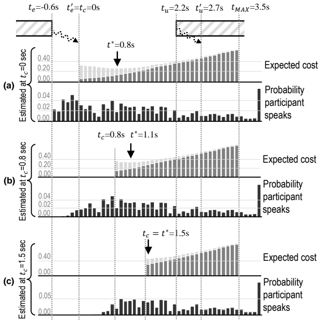
Figure 5. Decision-theoretic model avoiding undesirable gap.
