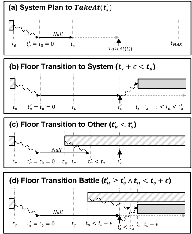
Figure 2. Illustrations of system plan to take the floor at time t'_s (a), and three possible outcomes (b,c,d).
