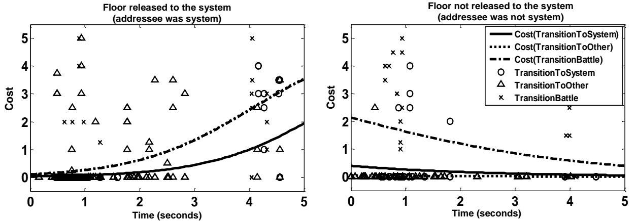
Figure 3. Estimating costs for actions over time from assessments.
