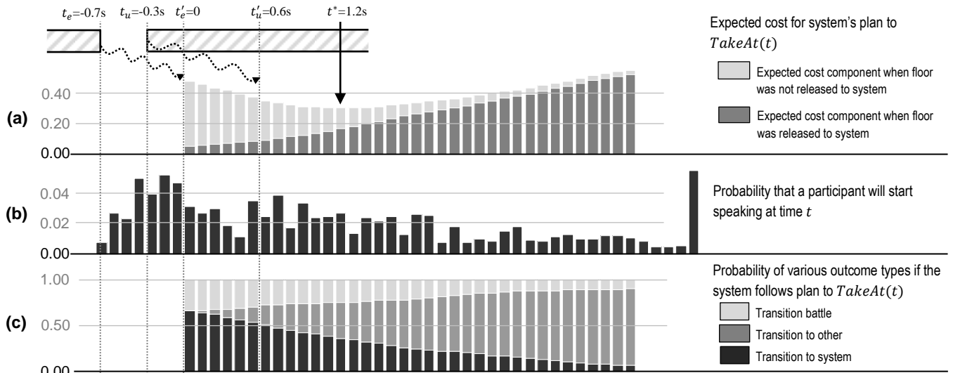
Figure 4. Decision-theoretic model avoiding floor conflict. (a) Expected cost for plan to TakeAt(t) , (b) probability distribution over time that the user will speak, and (c) inferred outcome-type probabilities for plan to TakeAt(t) .
